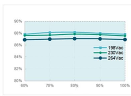
Fig.6 Efficiency-Load curve
