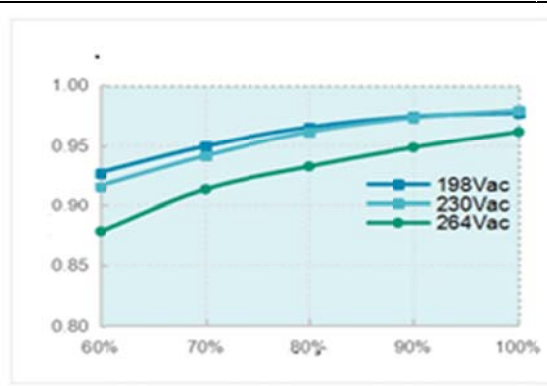
Fig.6 Efficiency-Load curve
