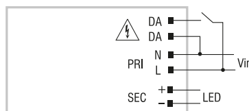
PUSH SWITCH diagram Collegamento PUSH SWITCH
