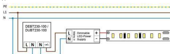
Typical connection scheme
