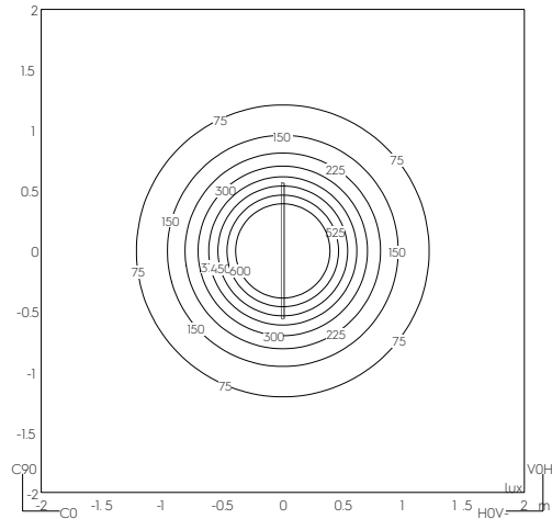
Room (m): 4x4x3m H luminaire (m): 2,5 Ref. surface: floor
